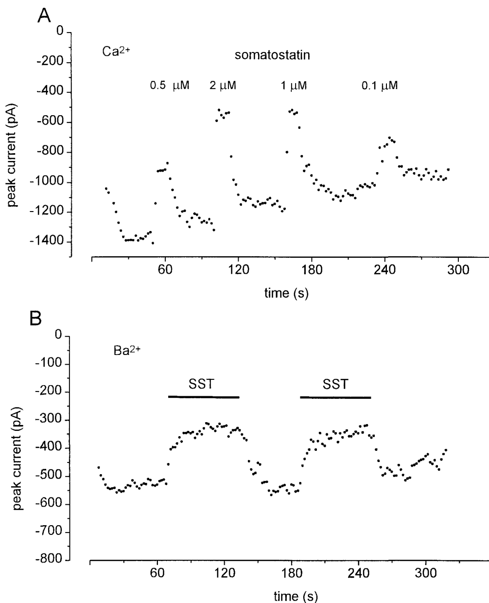
Fig. 3. Suppression of the peak currents by somatostatin. A: currents elicited in 15 mM \text{Ca}^{2+} were suppressed by SST in different concentrations. The duration of each SST application was 20 s. B: suppression of the currents in 15 mM \text{Ba}^{2+} by 1 \mu\text{M} SST. The duration of the SST application is indicated by bars.
